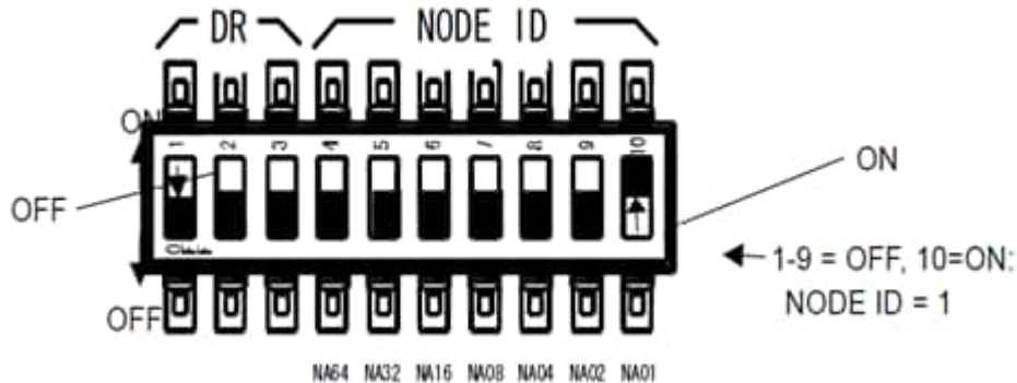
Figure 4.1 DIP Switch
